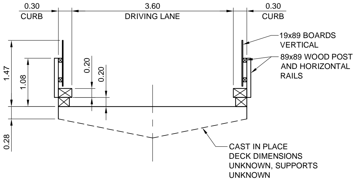
BRIDGE 08 - SECTION
