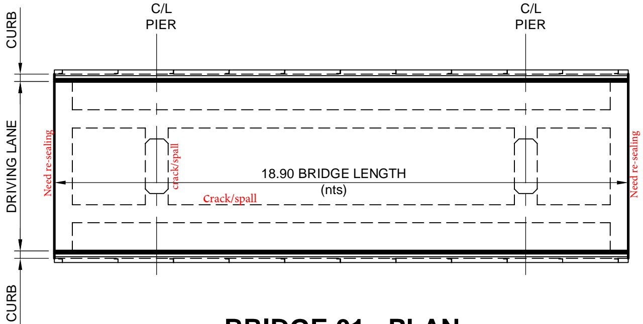
BRIDGE 01 - PLAN
