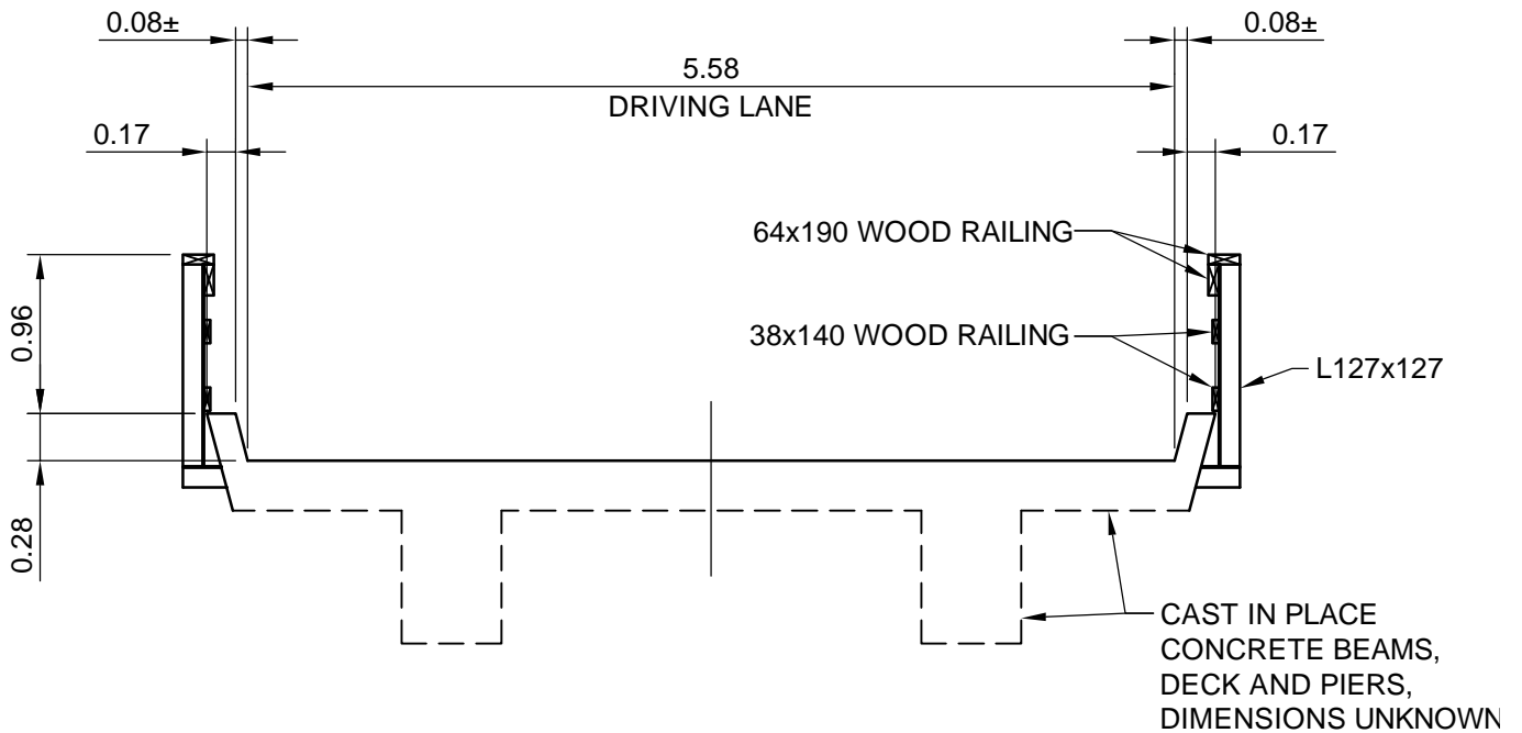
BRIDGE 01 - SECTION
